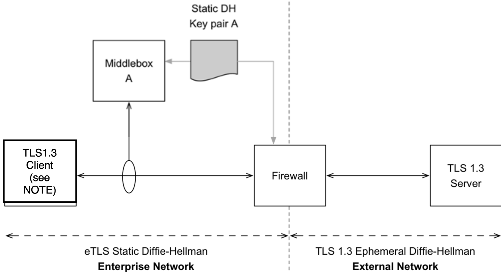
Figure 4.2: eTLS architecture with enterprise clients
